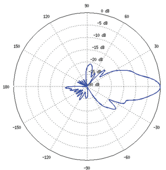
Horizontal Elevation
